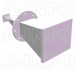
LB-28-25-A2SPO Standard Gain Horn Antenna 26.5-40GHz 25dB Gain Rectangular Waveguide Interface
