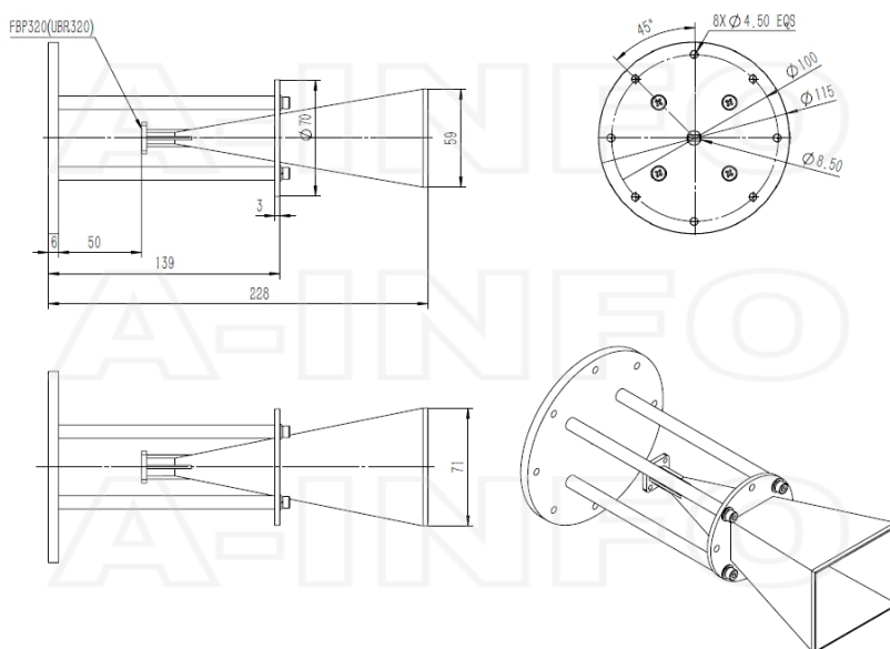
FBP320 Output with Round Mounting Bracket (Option, P/N: LB-28-25-MB2)
